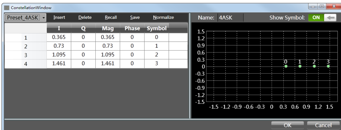
Figure 2-41 Custom modulation
