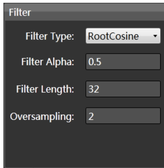
Figure 2-42 Filter interface
